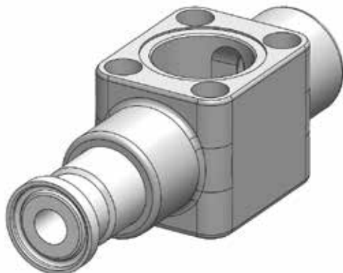
TRI-CLAMP
